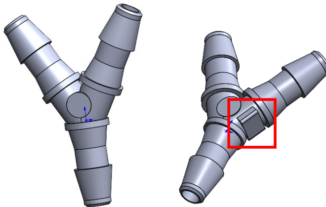
Image 1: Left – before adding shear gate. Right – after adding shear gate.
