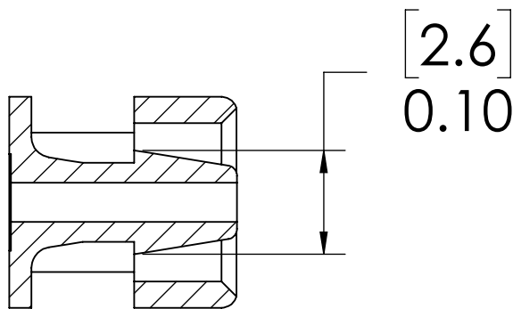
SECTION C-C
