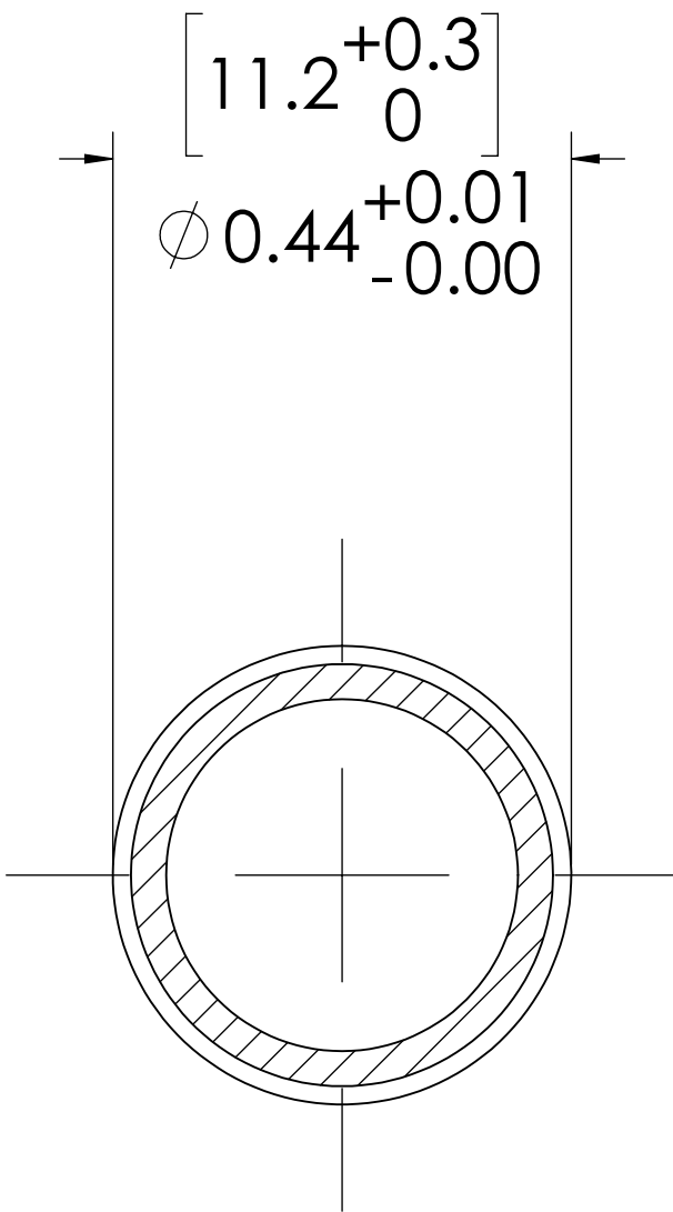
PANEL OPENING SECTION A-A
