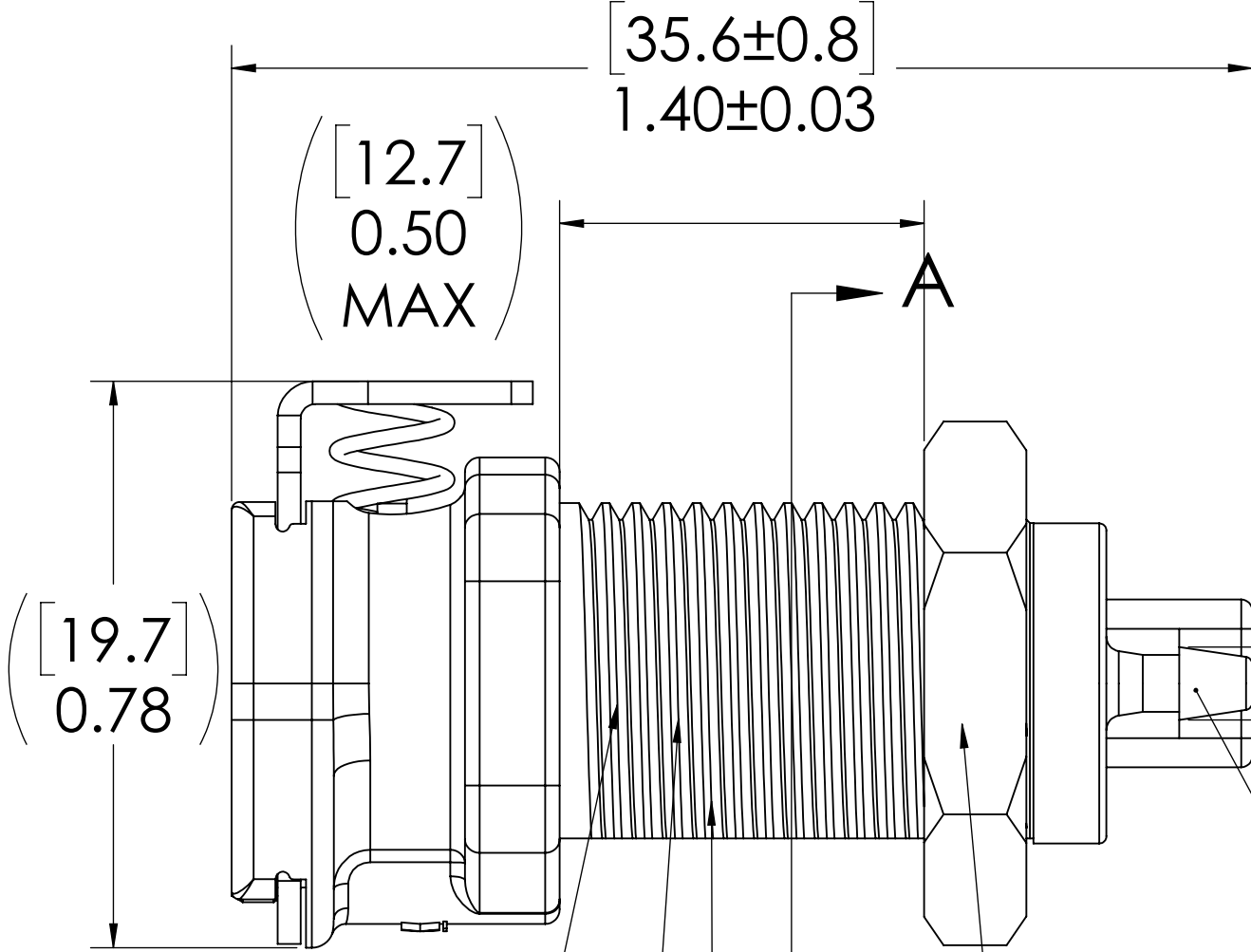
VALVE O-RING, INTERNAL (BUNA-N) VALVE SPRING, INTERNAL (STAINLESS STEEL)
