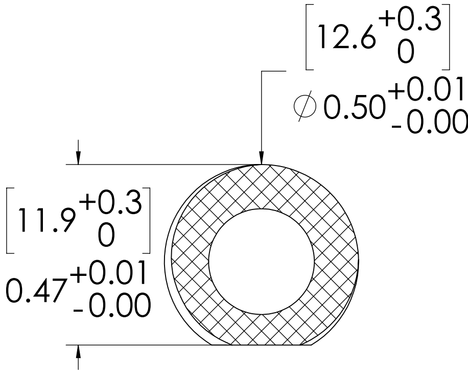
PANEL OPENING (SECTION A-A)
