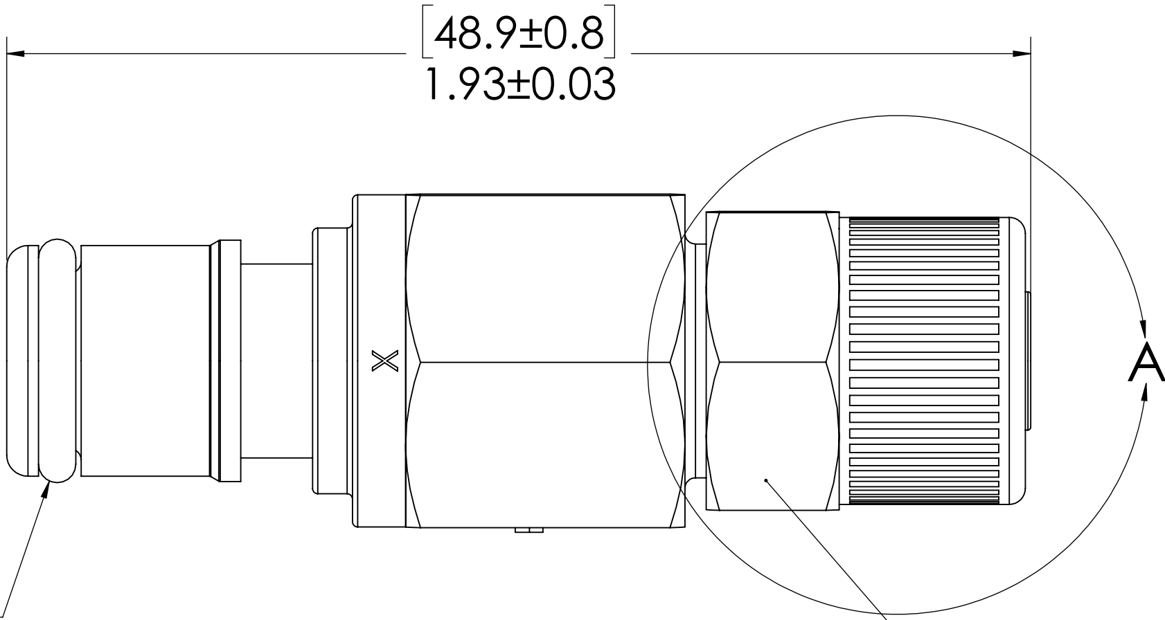
PTF NUT (BRASS, NICKEL PLATED) (PACKAGED SEPERATELY)
