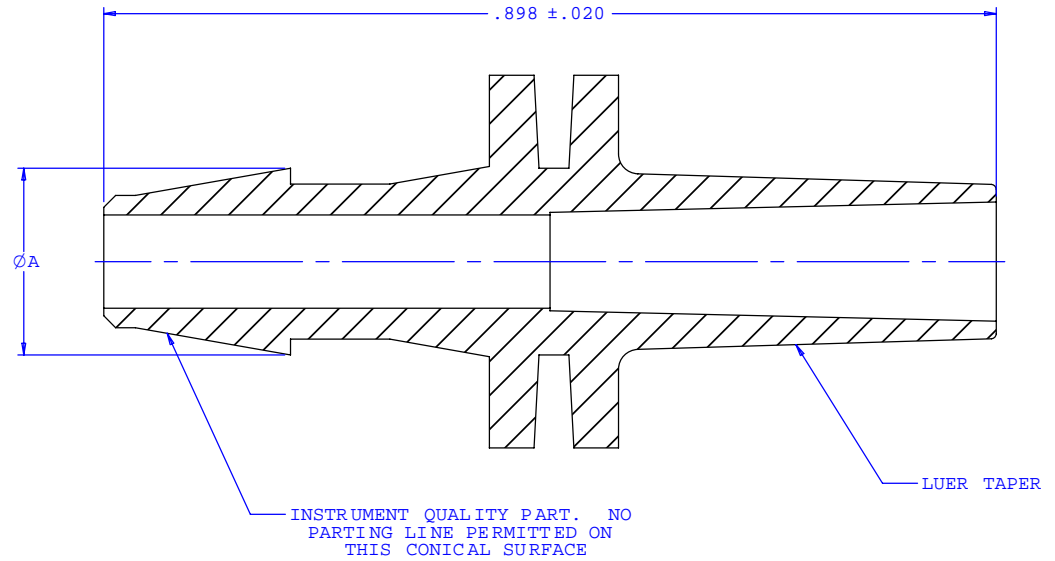
SECTION B-B
