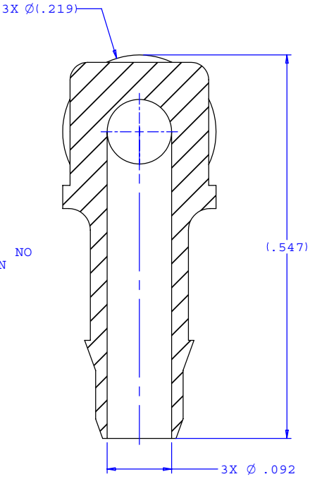
SECTION B-B
