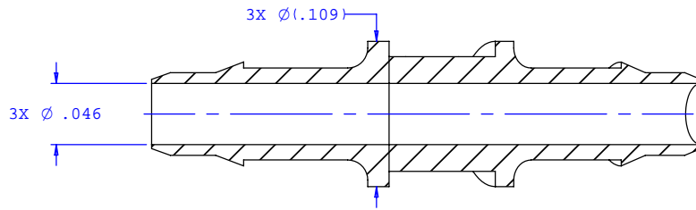
SECTION B-B
